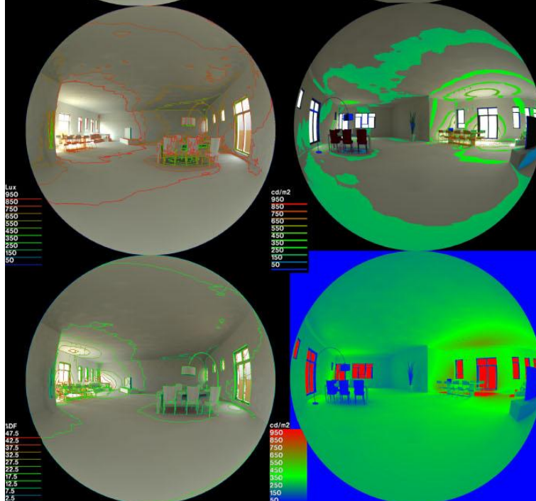
Simulation results displayed as colour images with different contour plots (Contour lines, Contour bands, False Color).
